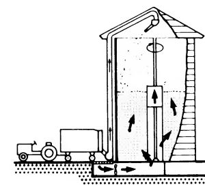
7 Hay tower: filling and ventilation
